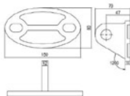
MQ-34 Material: SUS304/SUS316 Stainless Steel Finish: Satin/Polish/PVD
